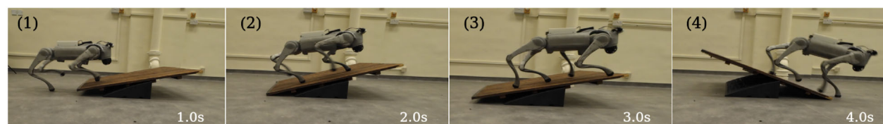
(b) Real-world dynamic balance control process of the Unitree Go2 robot on the Seesaw Board.
