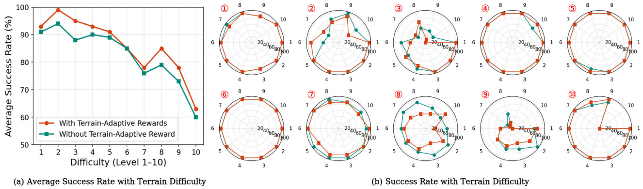
FIGURE 5 | Ablation of terrain-adaptive reward vs. fixed-weight reward. (a) Success rate vs. terrain difficulty level (1–10). (b) Performance by terrain difficulty level (1)–(10), with vs. without terrain-adaptive reward.
