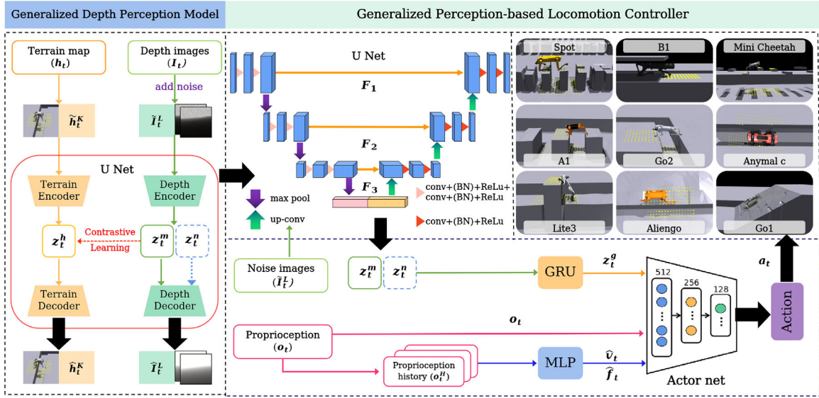
FIGURE 1 | The framework of the proposed MGDP. The architecture is composed of a Generalized Depth Perception Model and a Generalized Perception-Based Locomotion Controller. The perception model takes multi-modal inputs (depth map and height map) and extracts a highly generalized, low-dimensional terrain feature via contrastive learning. This model integrates an explicit depth map denoising mechanism and achieves an effective decoupling of terrain perception from robot dynamics. The locomotion controller combines this generalized feature with proprioceptive history to output the final joint torque commands. This decoupled design is critical for achieving the policy's superior cross-terrain generality and fast platform transferability.
