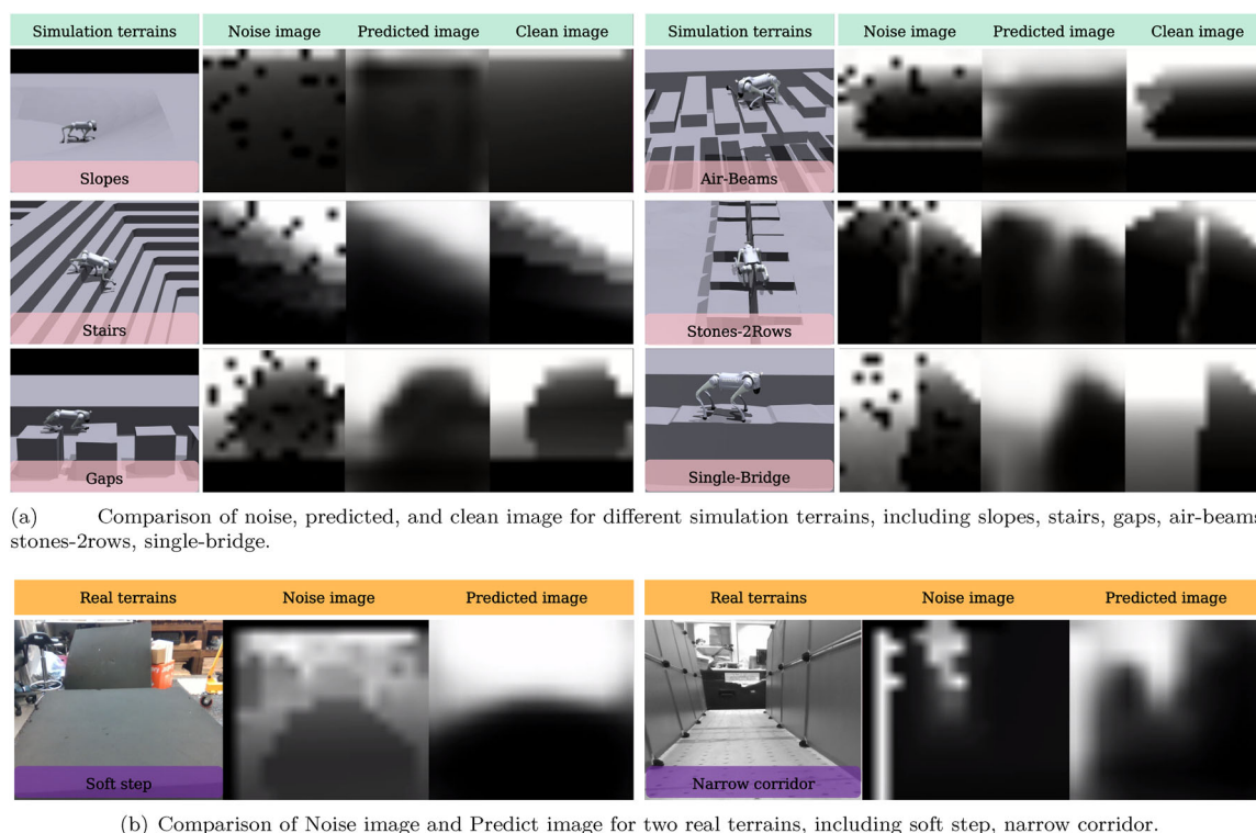
FIGURE 8 | Image denoising and reconstruction results on simulation and real terrains.
