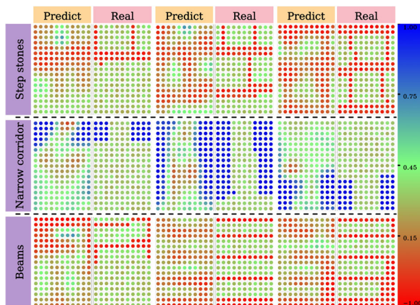
FIGURE 9 | Comparison of predicted and real height maps across different terrains (step stones, narrow corridor, beams) at different time steps.
