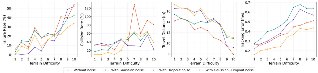
FIGURE 4 | Ablation of depth noise on locomotion performance. The figure compares four training conditions (without noise, Gaussian, Dropout, Gaussian+Dropout) across 10 different terrain difficulty levels using four evaluation metrics: (a) failure rate (%), (b) collision rate (%), (c) travel distance (m), and (d) tracking error (m/s).
