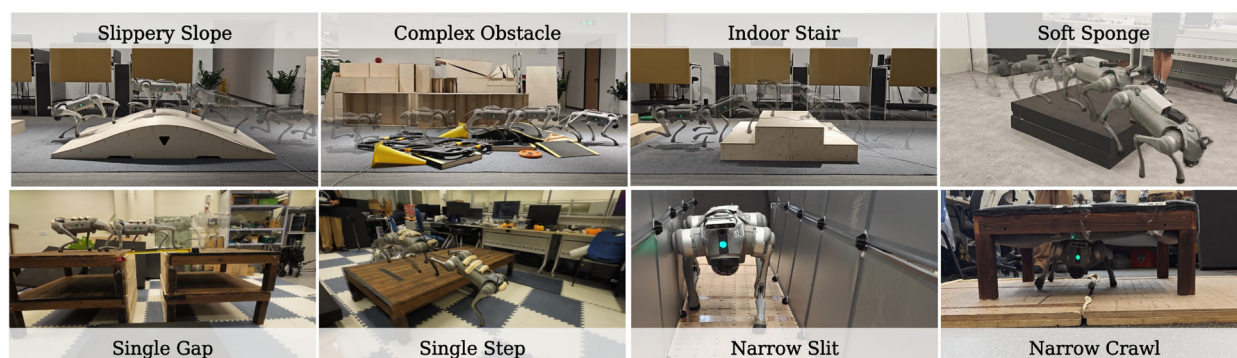
(a) Real-world deployment of the Unitree Go2 robot on diverse indoor terrains, including slippery slope, complex obstacle, indoor stair, soft sponge, single gap, single step, narrow slit, and narrow crawl.
