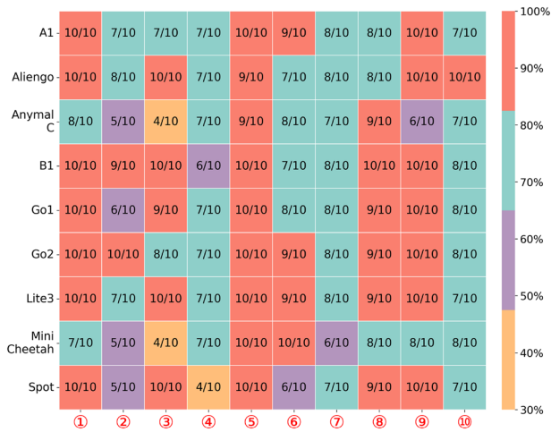
FIGURE 6 | Comparison of terrain traversal performance among 9 quadruped robots across 10 types of extreme terrains. Each cell displays the ratio of the maximum difficulty that a robot can stably traverse to the greatest difficulty of the corresponding extreme terrain.
